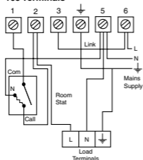
1) Control of Heating Function only (Mains Voltage)
